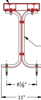
CONCRETE ANCHORED OPTION SEE DETAIL "3"
